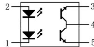
Internal Circuit
